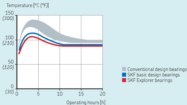
Diagram 1 Typical temperature behaviour of tapered roller bearings during the running-in period (approximate values)
