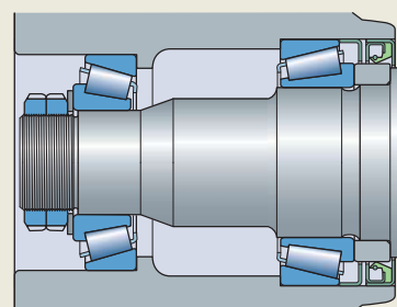
Single bearings mounted back-to-back
